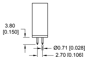
Size 22 contacts
