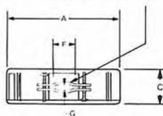
CABLE CLAMP CONFIGURATION FOR SIZES 9, 15 AND 25
