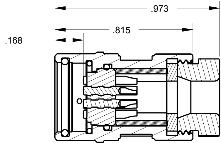
SECTION Z-Z
