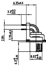
Shell size 1-4
