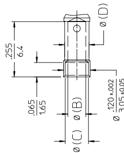
CRIMP
