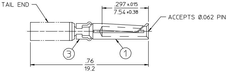
2 PIECE SOCKETS
