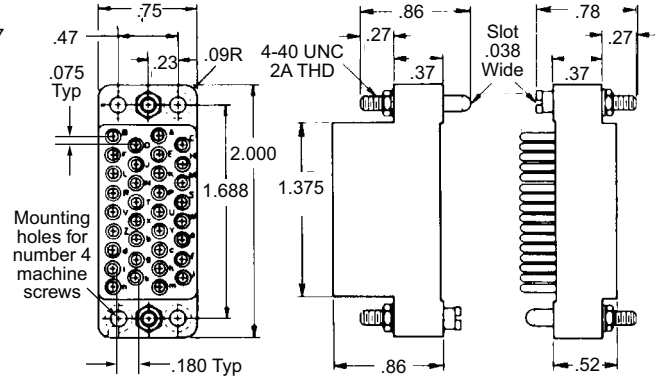
MRAC 34S-G
