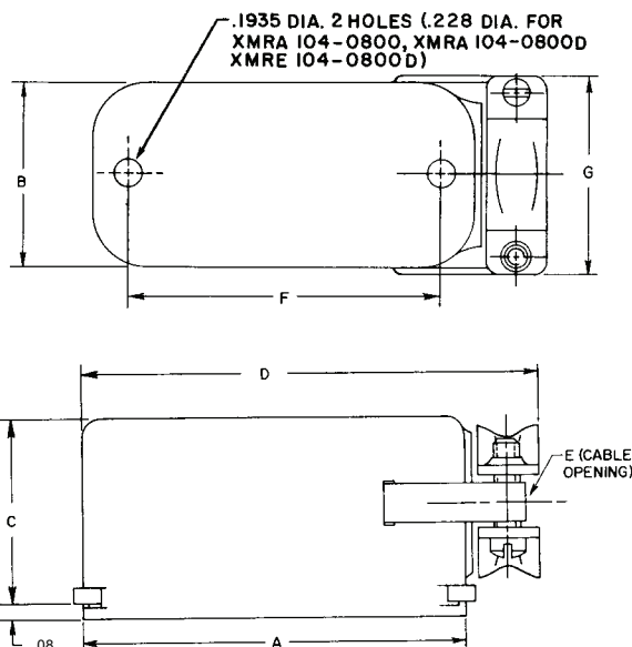
Side Cable Opening
