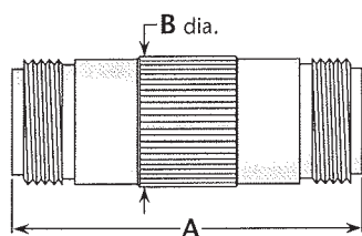
Figure 1 (Straight jack-jack; connects two plugs)
