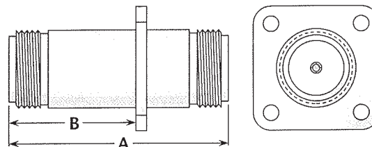
Figure 2 (Panel mount)
