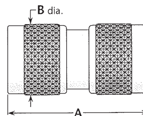
Figure 2 (Straight plug-plug; connects two jacks)
