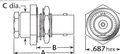
Figure 1 (Rear mount)
