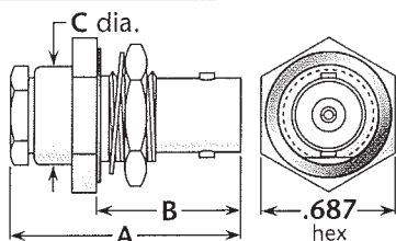
Figure 1 (Rear mount)
