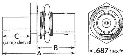
Figure 1 (Rear mount)
