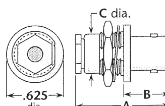
Figure 4 (Front mount)
