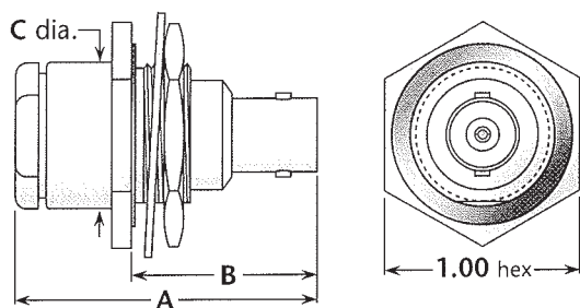
Figure 1 (Rear mount)
