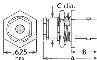
Figure 3 (Front mount)
