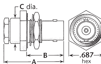
Figure 2 (Rear mount)
