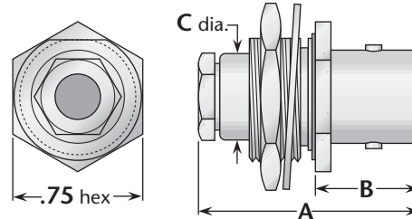
Figure 2 (Front mount)
