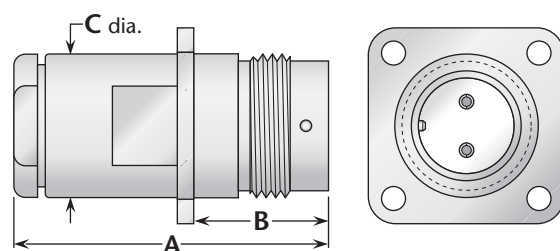
Figure 2 (Panel jack)
