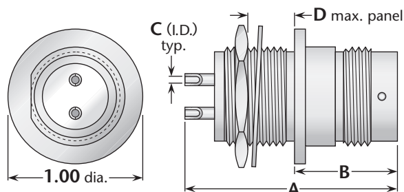
Figure 1 (Bulkhead jack receptacle, front mount)
