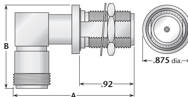
Figure 3 (Bulkhead mounted right angle jack-jack; connects two plugs)
