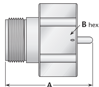
Figure 3 (Straight LC jack-large LC plug; connects one LC plug and one large LC jack)
