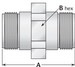
Figure 1 (Straight jack-jack; connects two plugs)
