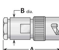
Figure 3 (Military clamp)
