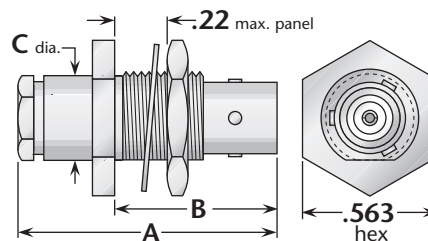
Figure 2 (Rear mount, wedge clamp)
