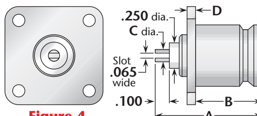
Figure 4 (Slotted contact)
