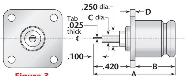
Figure 3 (Tab contact)
