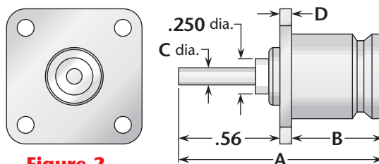
Figure 2 (Post contact)
