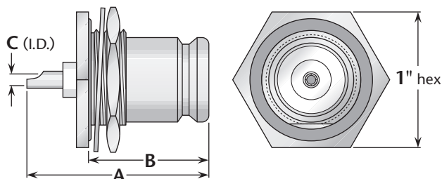
Figure 1 (Rear mount, with mounting gasket)
