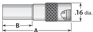
Figure 1 (Crimp type for flexible cable)
