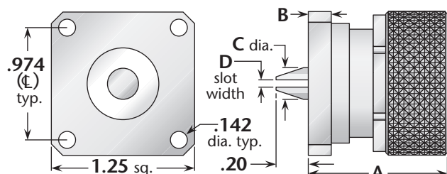
Figure 1 (Standard flange)
