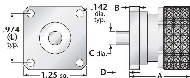
Figure 1 (Standard flange)
