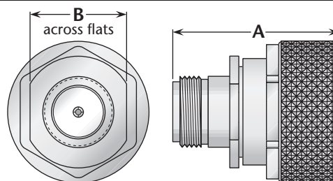
Figure 2 (7/16 plug-N jack)
