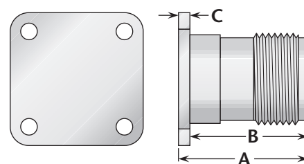
Figure 4 (Dummy receptacle)
