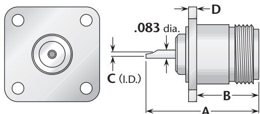
Figure 1 (Straight jack receptacle)
