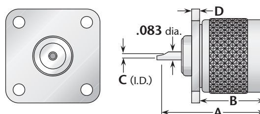
Figure 2 (Straight plug receptacle)
