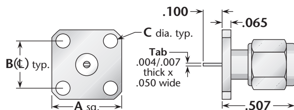
Figure 2 (1/2" square flange)
